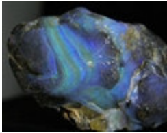
Opal, Windorah, Queensland, Australia.
