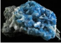
Cavansite, Wagholi, Poona India.
