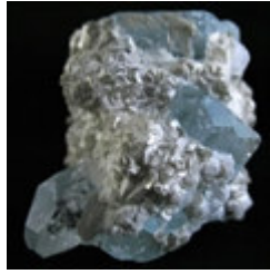
Aquamarine, albite, muscovite, with schorl inclusions, Shigar, North West Frontier Province, Pakistan.
