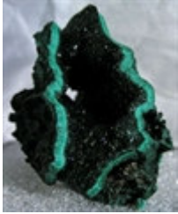
Malachite, Kolwezi, Katanga Province, Congo.
